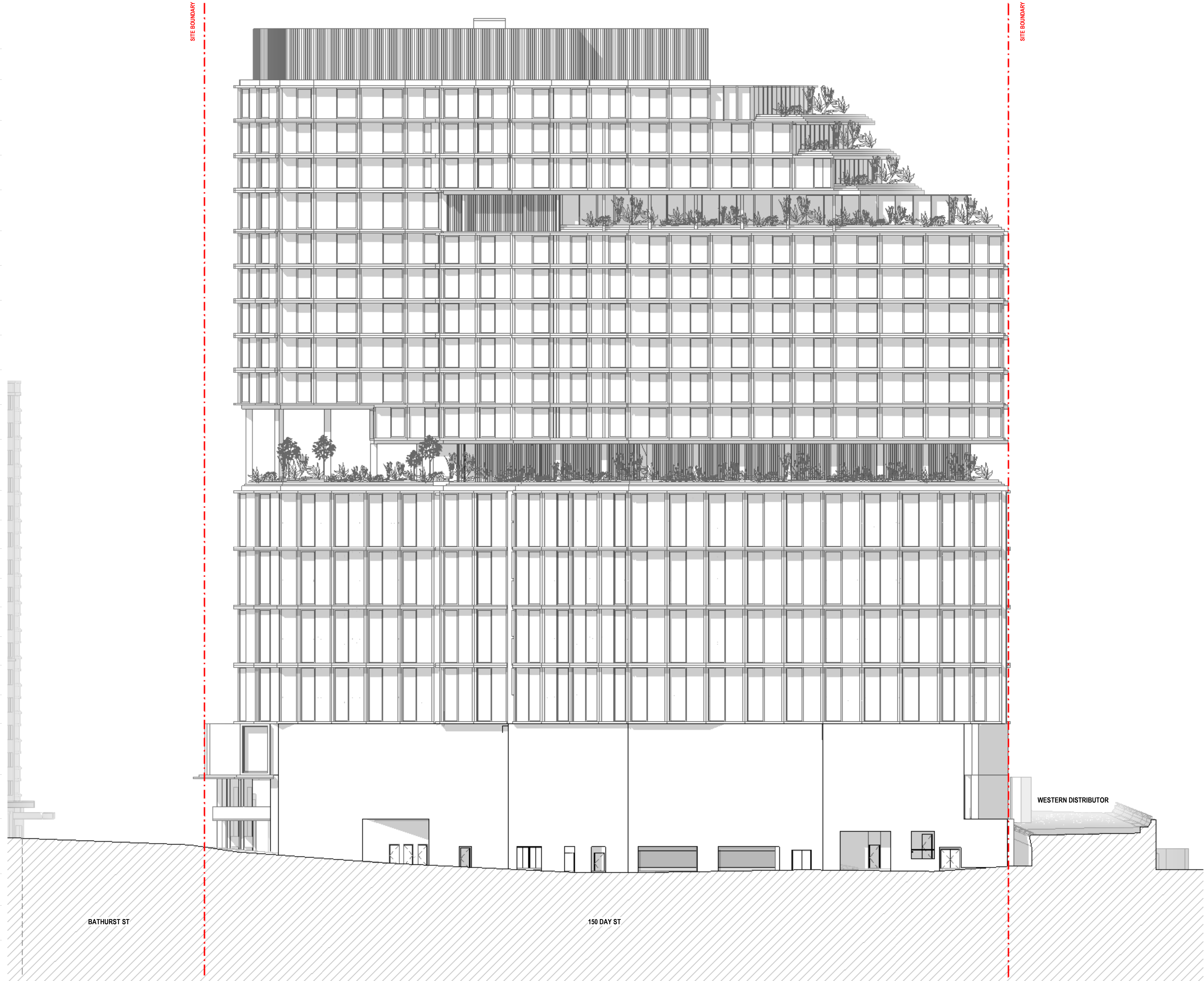
1 PROPOSED EAST ELEVATION - SANDS ST DD_501 1:200
